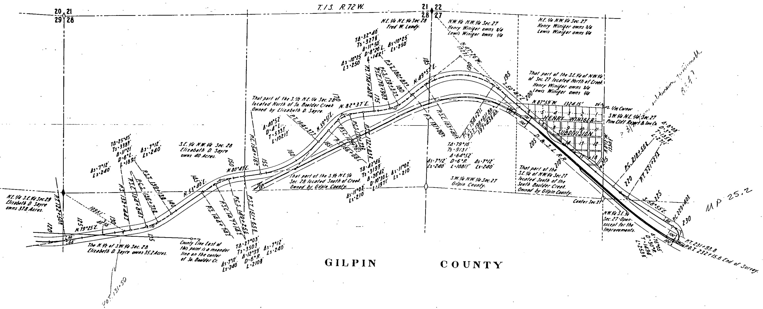
RIGHT OF WAY MAP COAL CREEK HIGHWAY COLO. 31 STA. 120+00 TO STA. 232+15.6
