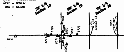
Monumentation Detail (NOT TO SCALE)
