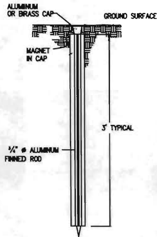
TYPE 1 MONUMENT
