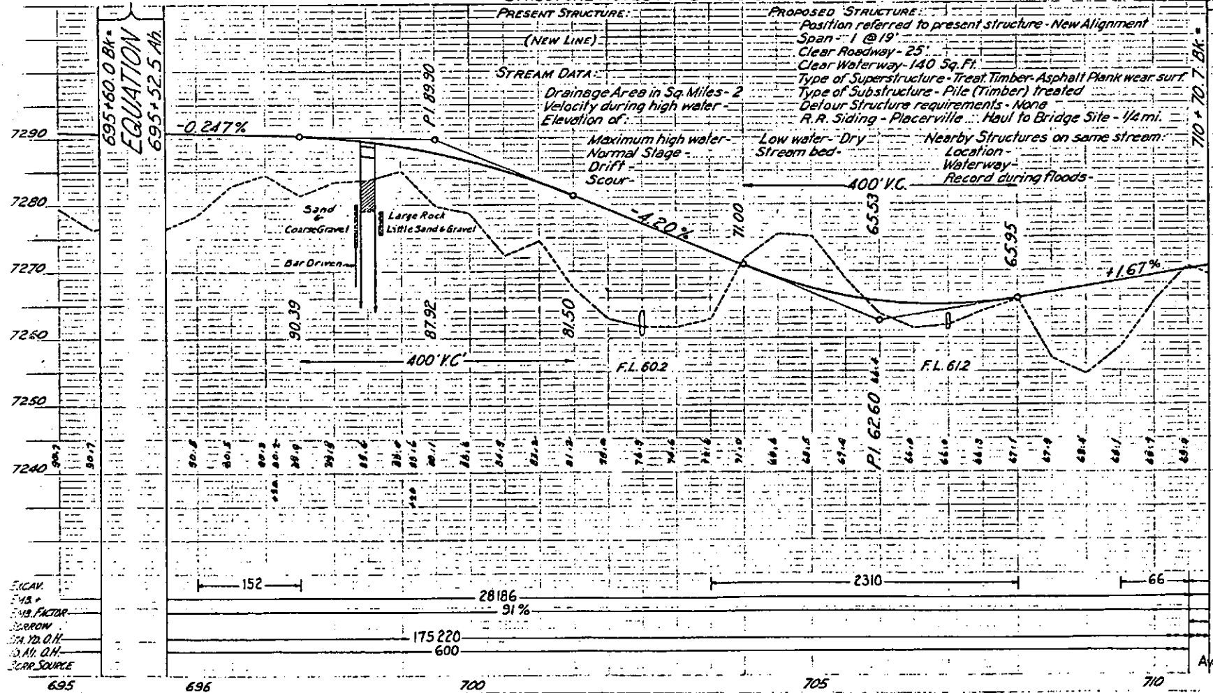
STRUCTURE NOTES FOR BRIDGE STA. 698+40 TO 698+60.5 STRUCTURE NO. L-4-J
