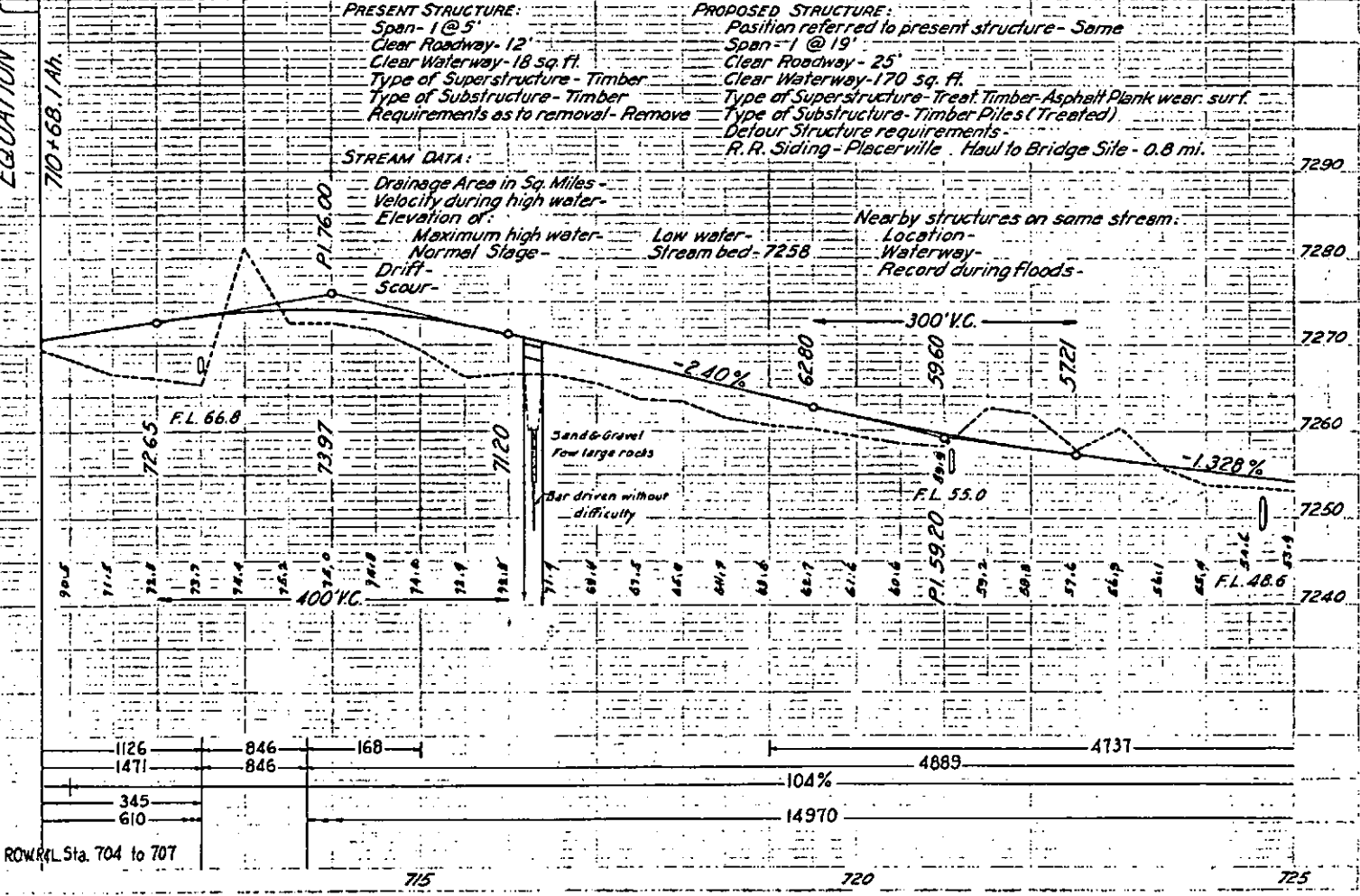
STRUCTURE NOTES FOR BRIDGE STA. 716+20 TO 716+40.5 STRUCTURE NO. L-4-H
