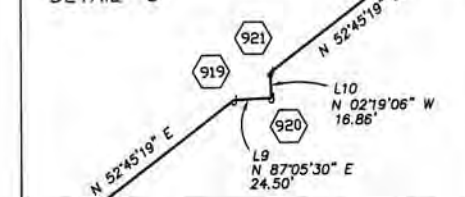
DETAIL "C"
