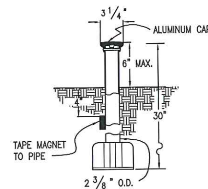
TYPE 3 MONUMENT
