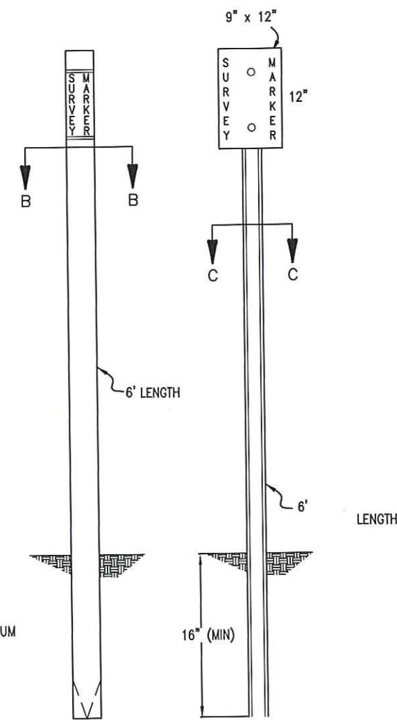
WITNESS POSTS
