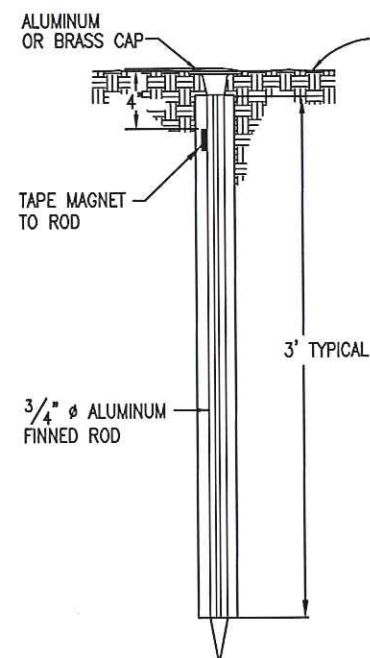
TYPE 1 MONUMENT
