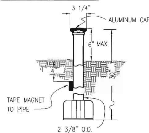
TYPE 3 MONUMENT
