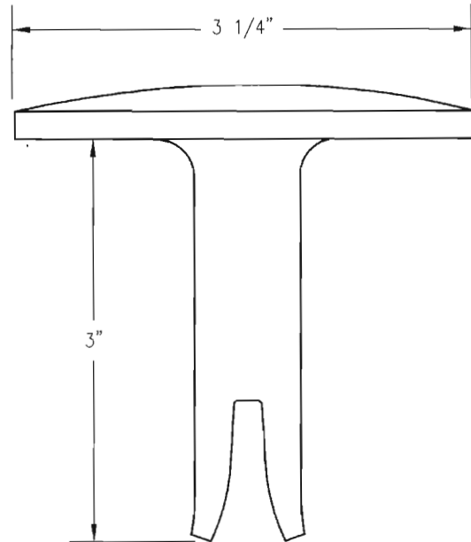
ALUMINUM CAP
