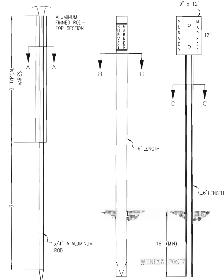
TYPE 2 MONUMENT
