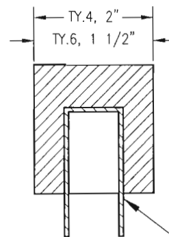
ALUMINUM CAP
